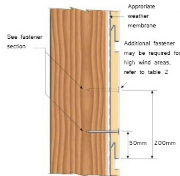
Figure 2: Concealed Fixing Detail
