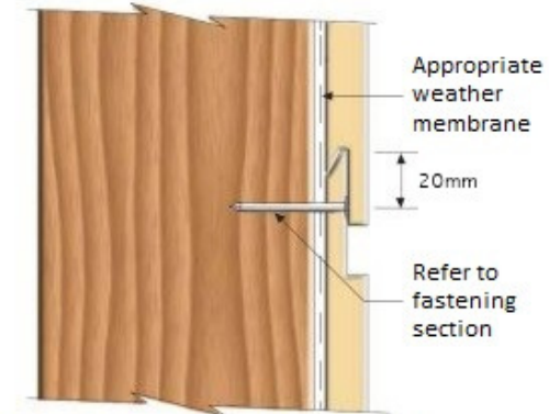
Figure 2: Concealed Fixing Detail
