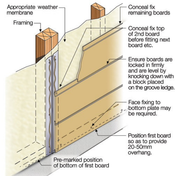
Figure 1: Board Installation (internal lining omitted for clarity)
