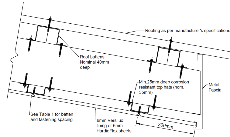
Figure 1: Soffit / Eaves w Metal Fascia
