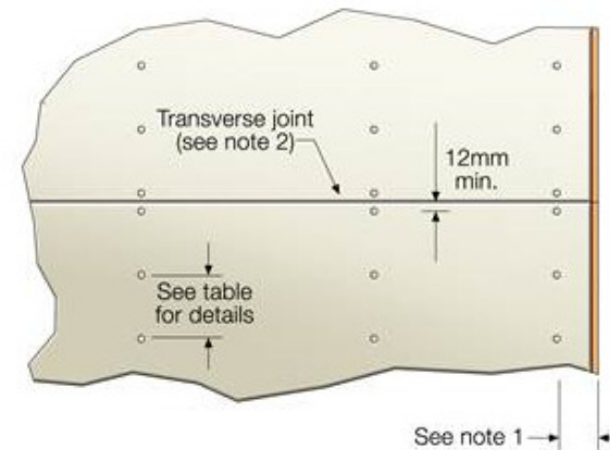
Figure 3: Plan View of Eaves / Soffit Layout
