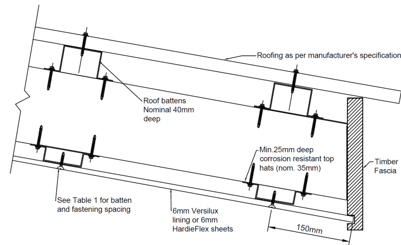
Figure 2: Soffit / Eaves w Timber Fascia
